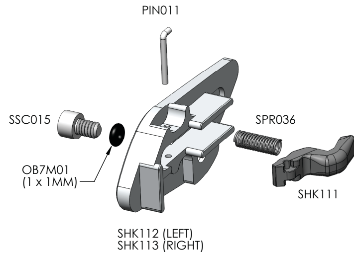
BALL DETENT
